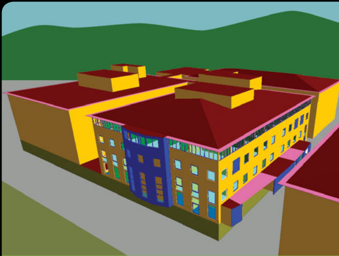
St. George's Hospital Stage 2 Rebuild detailed energy model
